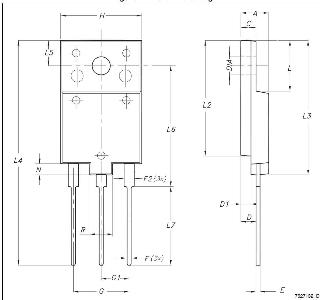
Figure 24. TO-3PF drawing
