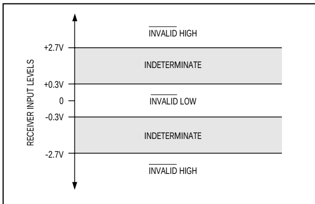
Figure 7. Receiver Positive/Negative Thresholds for \overline{INVALID}
