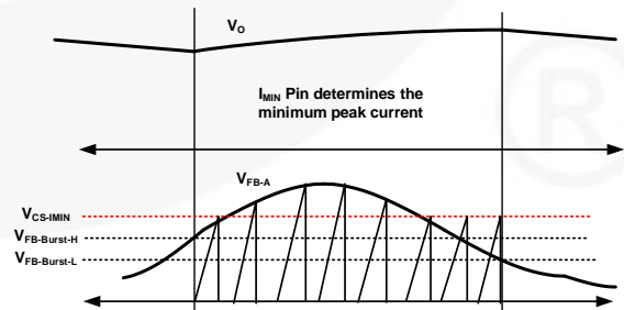
Figure 31. Burst-Mode Operation with IMIN
