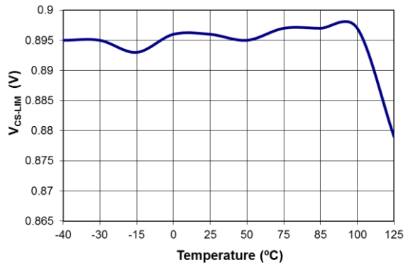
Figure 18. Current Limit Threshold Voltage (V CS-LIM ) vs. Temperature
