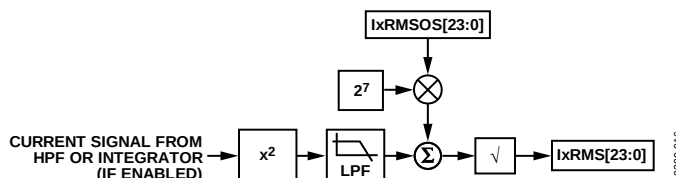
Figure 32. IxRMS Signal Path
