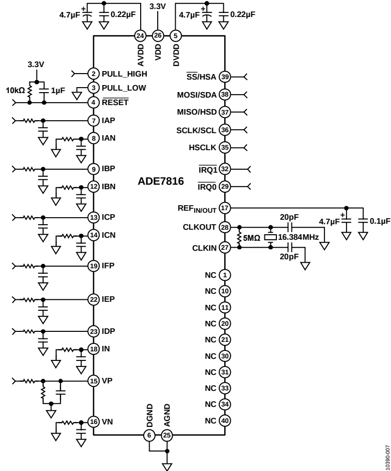
Figure 22. Test Circuit
