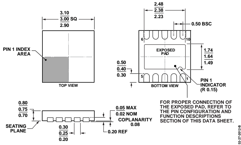
FOR PROPER CONNECTION OF THE EXPOSED PAD, REFER TO THE PIN CONFIGURATION AND FUNCTION DESCRIPTIONS SECTION OF THIS DATA SHEET. Figure 49. 10-Lead Lead Frame Chip Scale Package [LFCSP_WD] 3 mm x 3 mm Body, Very Very Thin, Dual Lead (CP-10-9) Dimensions shown in millimeters
