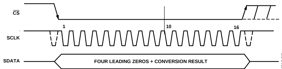
Figure 19. Normal Mode
