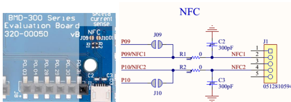
Figure 13 – NFC Connector
