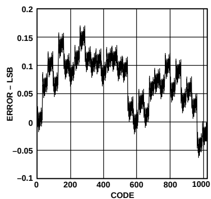
Figure 12. Typical INL
