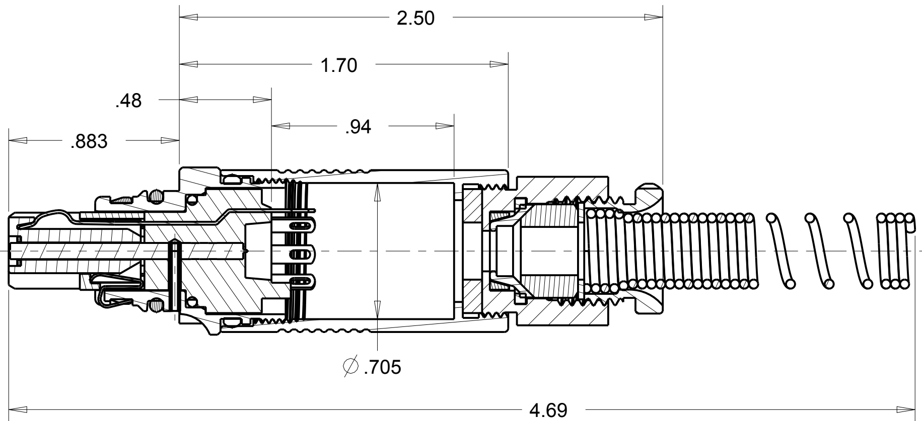
SECTION Z-Z
