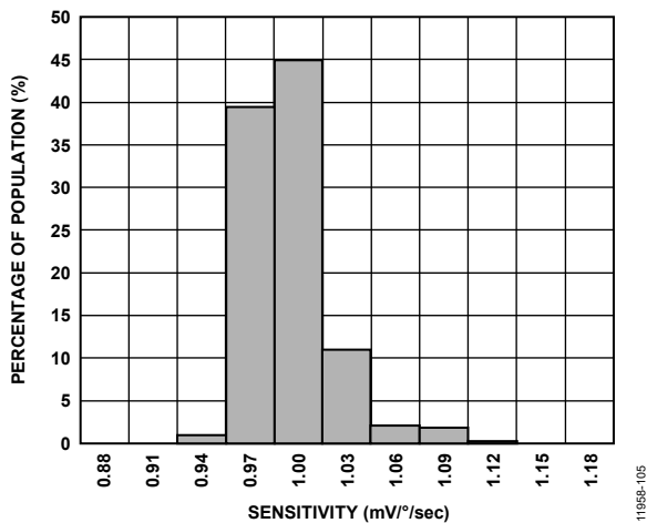
Figure 6. Sensitivity at 25°C
