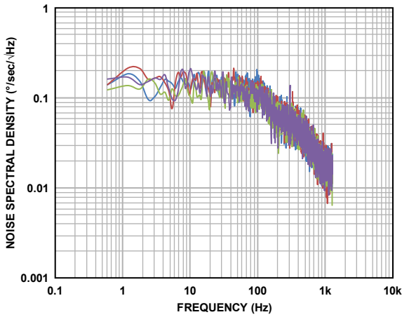
Figure 18. Typical Noise Spectral Density ( C_{OUT} = 0.01\text{ }\mu\text{F} )
