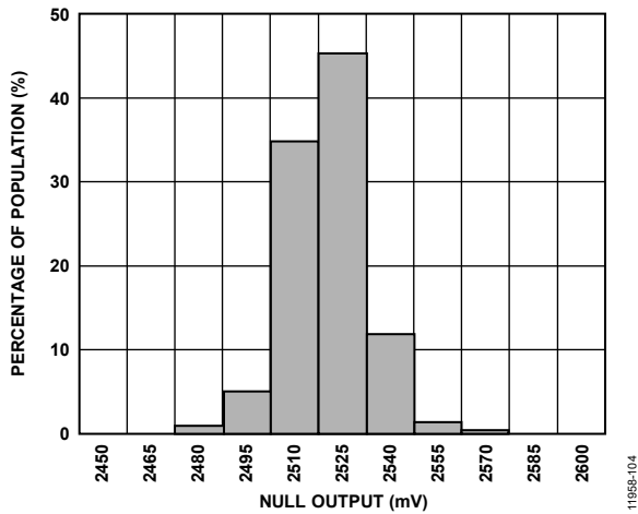
Figure 5. Null Output at 25°C
