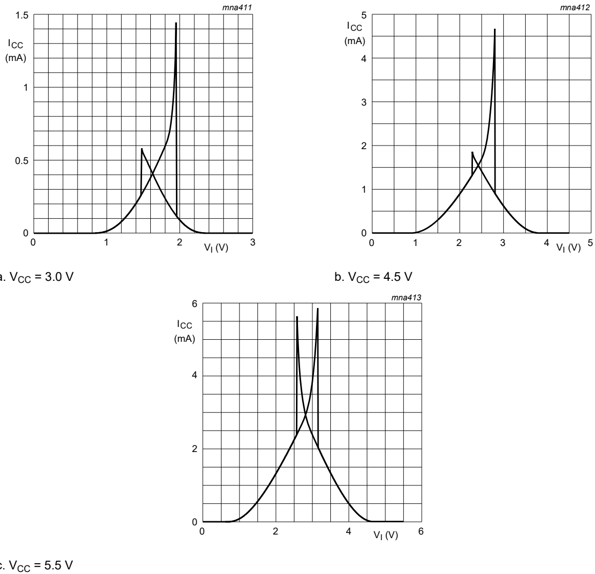
Fig. 10. Typical 74AHC132-Q100 transfer characteristics
