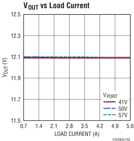
Figure 3. Load Regulation
