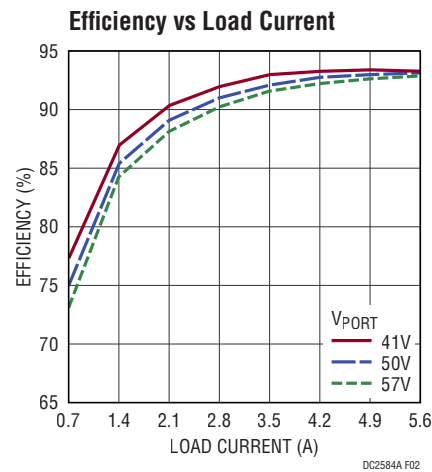
Figure 2. Efficiency (End-to-End)
