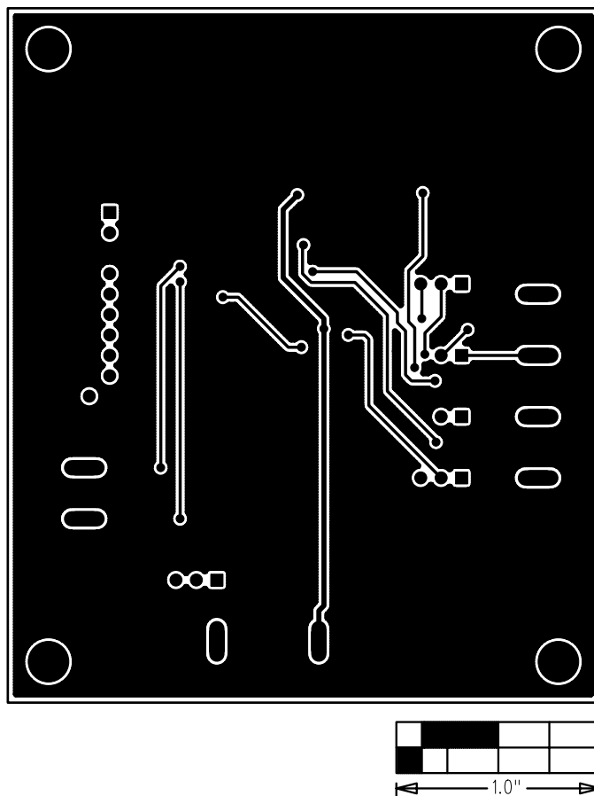
Figure 6. MAX7307 EV Kit PCB Layout—Solder Side
