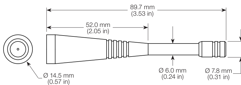
Figure7. CW LTE Band 20 Antenna Dimensions
