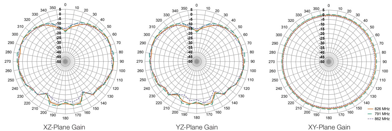
Figure9. Radiation Patterns for CW LTE Band 20 Antenna
