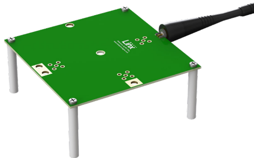
Figure 8. CW LTE Band 20 Antenna Shown On Edge of Evaluation Board
