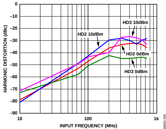
Figure 49. ADV3222 Harmonic Distortion, R_L = 100 \Omega , C_L = 4 \text{ pF}
