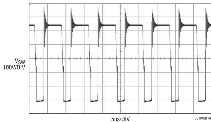
Figure 8. V IN = 277VAC
