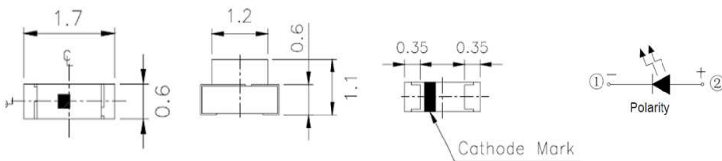
Figure 2. IN-S63AS Package Dimensions
