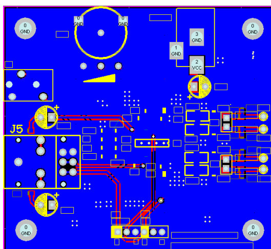
Figure 3: Bottom Layer
