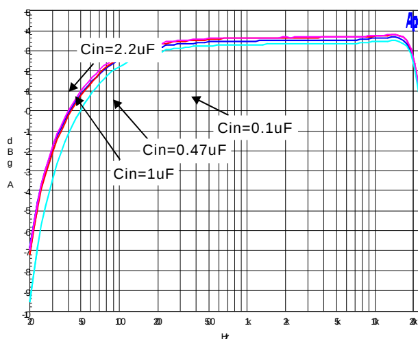
7. Frequency Response
