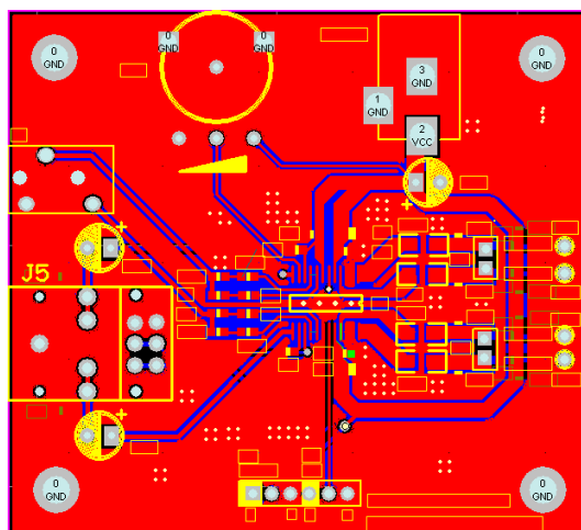
Figure 2: Top Layer
