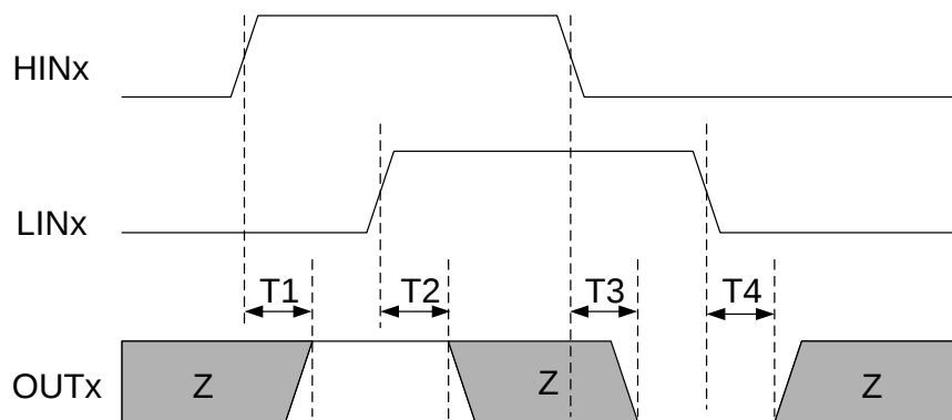
Figure 1: Input/Output Timing Diagram
