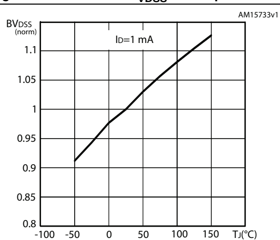
Figure 7. Normalized B VDS vs temperature
