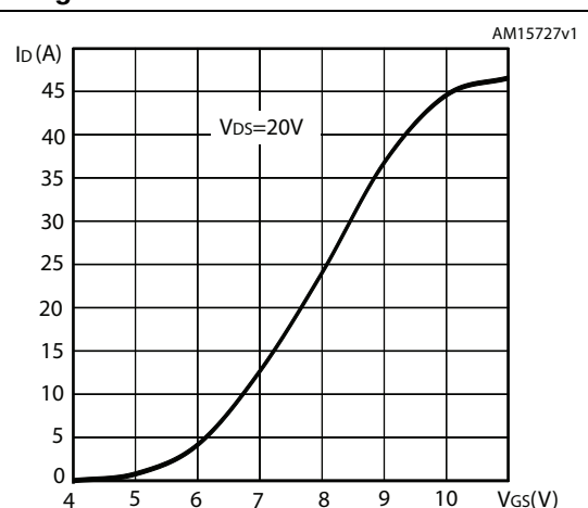
Figure 11. Transfer characteristics
