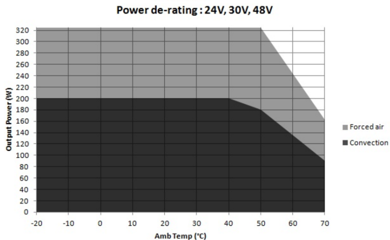
Figure 1. Derating Curves
