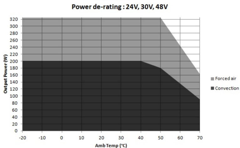
Figure 1. Derating Curves
