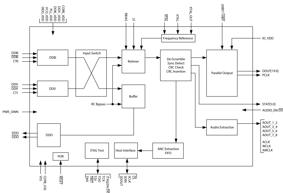
GS3470 Functional Block Diagram
