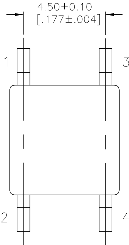
TERMINAL NUMBERS
