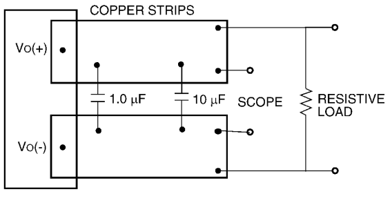
Figure 12. Input Reflected Ripple Current Test Setup.
