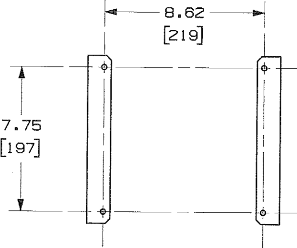
BENCH MOUNTING HOLE PATTERN
