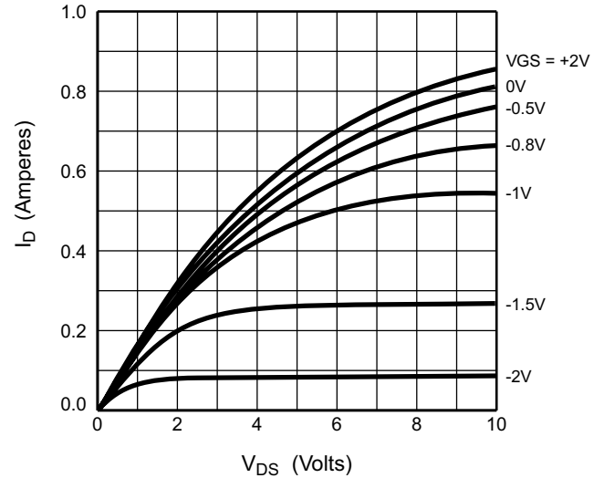
Saturation Characteristics
