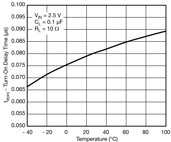
Figure 19 - Turn-On Delay Time vs. Temperature
