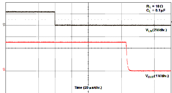
Figure 28 - SiP32453 Turn-Off Time ( V_{IN} = 2.5 \text{ V} )
