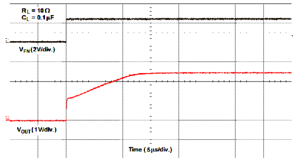
Figure 26 - Turn-On Time ( V_{IN} = 2.5 \text{ V} )
