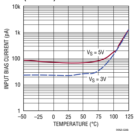
Input Bias Current vs Temperature (LTC2050)
