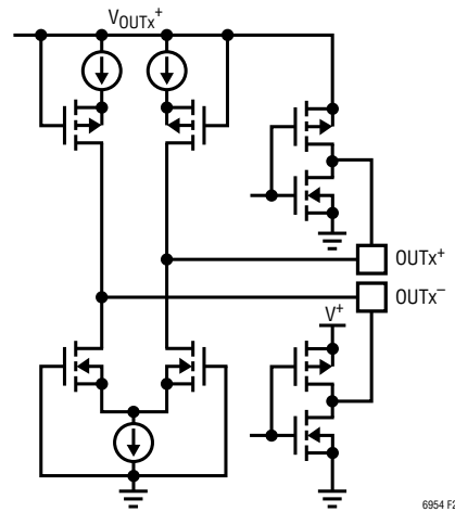
Figure 23. Simplified LVDS/CMOS Output Schematic (CMOS Mode, LVDS Circuit Shutdown)
