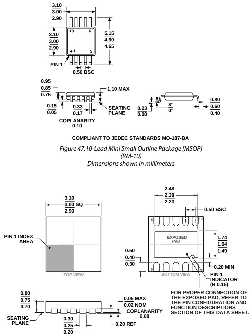
Figure 48. 10-Lead Lead Frame Chip Scale Package [LFCSP_WD] 3 mm × 3 mm Body, Very Very Thin, Dual Lead (CP-10-9) Dimensions shown in millimeters
