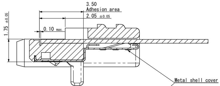
SEC. A-A(S=10/1)
