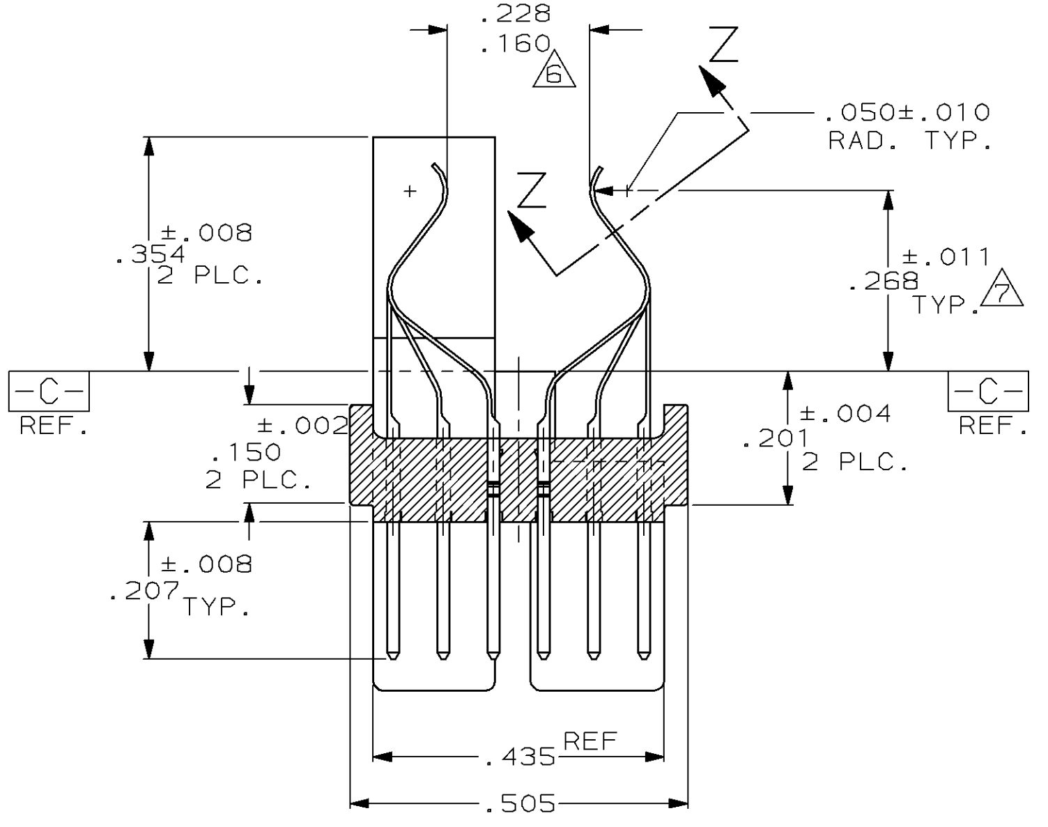
SECTION W-W SCALE 5:1 ROTATED CCW 90° (445269-1 ONLY)
