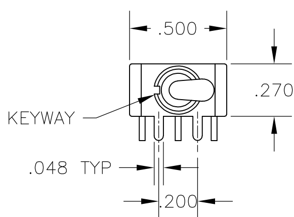
A RIGHT ANGLE 5
