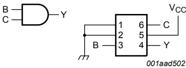
Figure 6. 2-input AND gate
