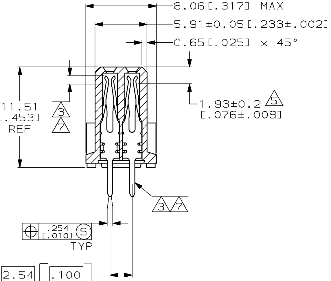
SECTION X-X
