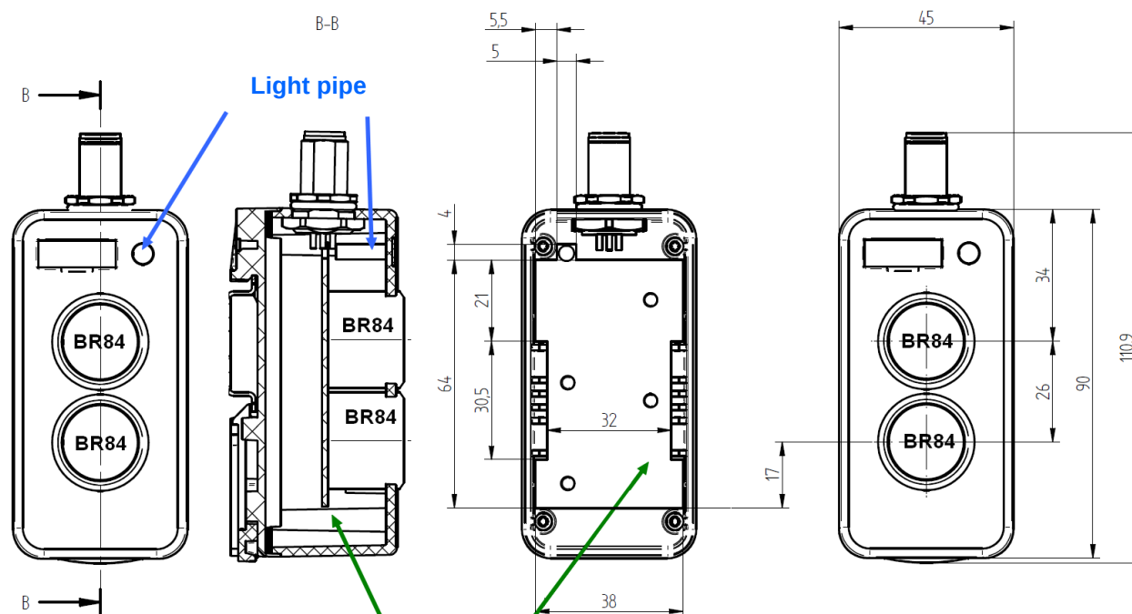
Dimensional diagram 1
