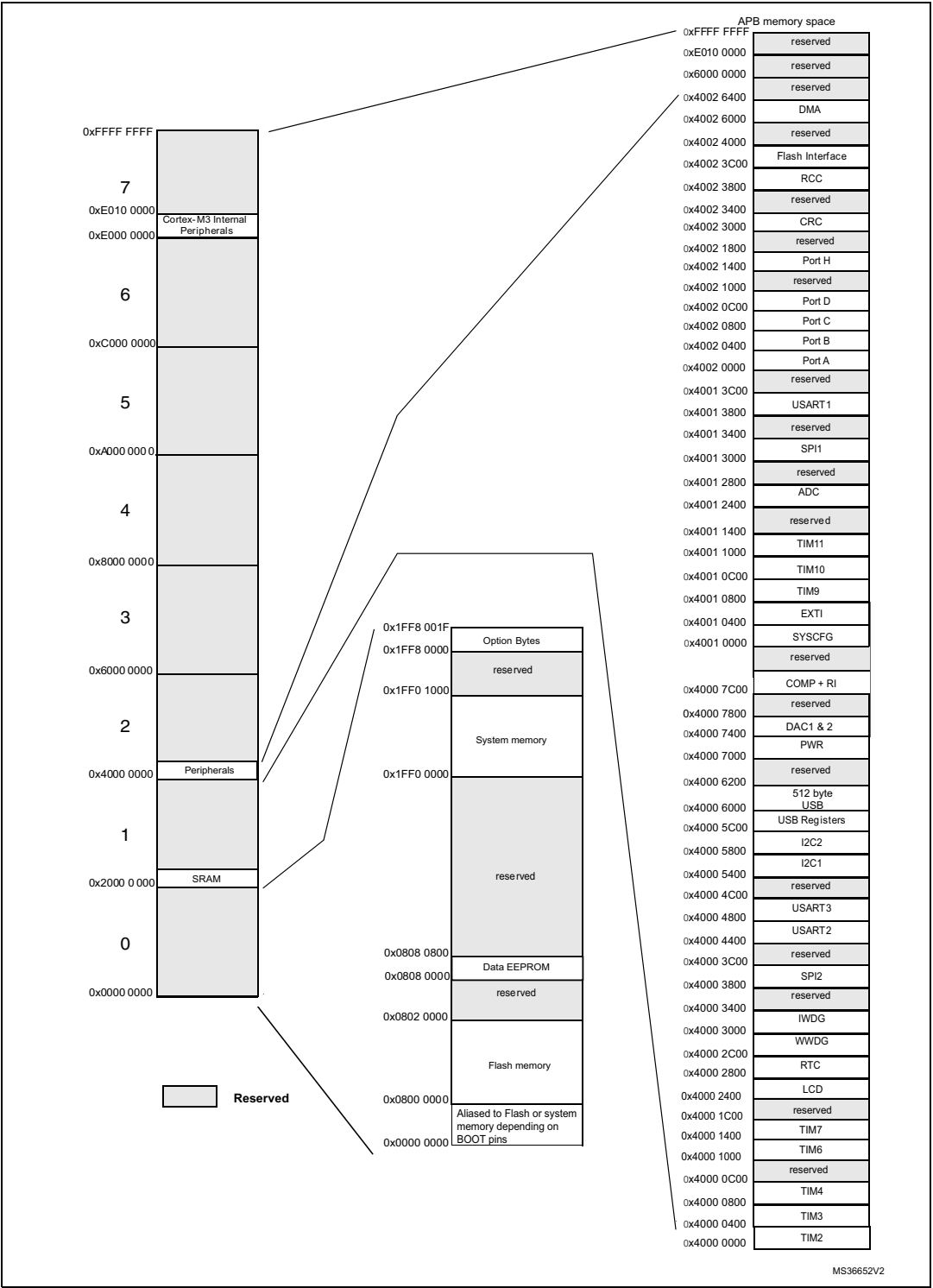
Figure 5. Memory map
