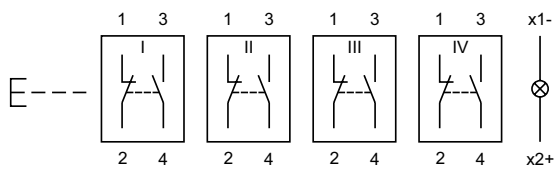
Wiring diagram 22
