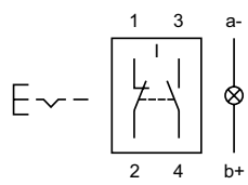
Wiring diagram 25
