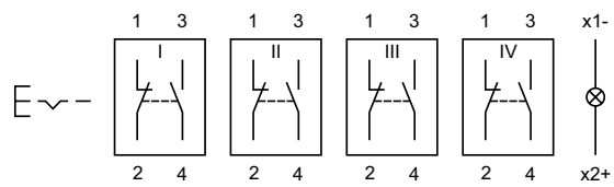
Wiring diagram 23
