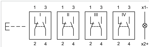
Wiring diagram 22
