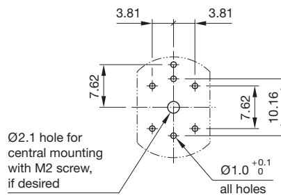
Component layout 2
