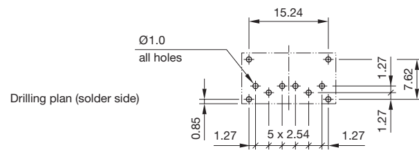
Component layout 3
