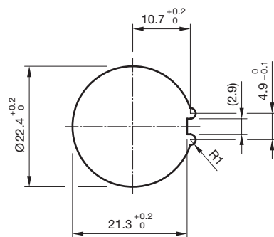
Mounting cut-outs 1
