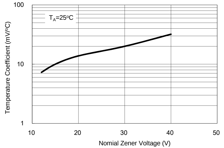
Fig. 2 Temperature Coefficient
