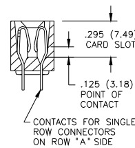
SECTION THROUGH CONTACT POSITION
