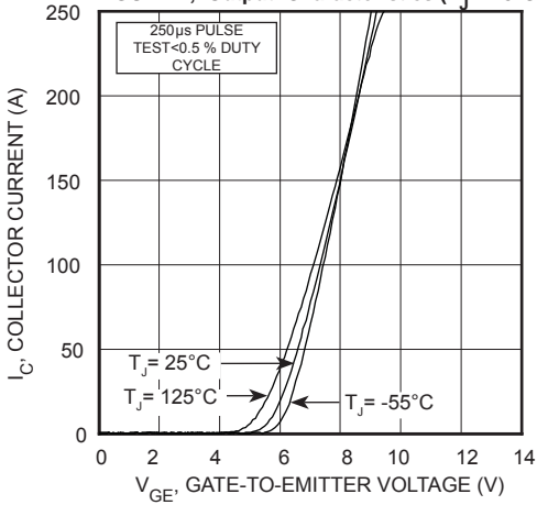
FIGURE 6, Transfer Characteristics
