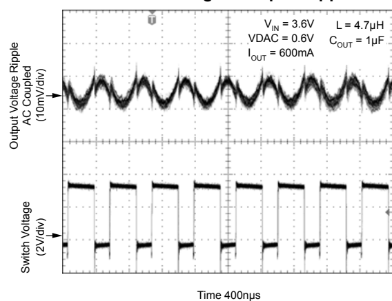
Switch Voltage - Output Ripple
