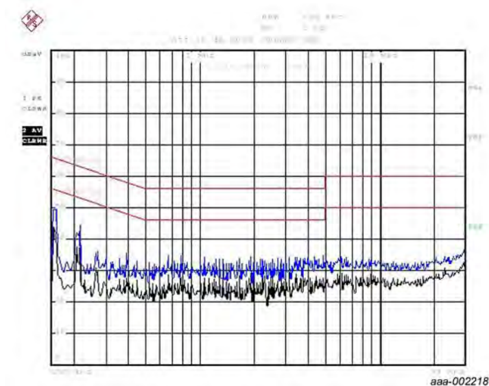
a. EMI at 115 V (AC) input voltage and 2 W output at 80 % load.
