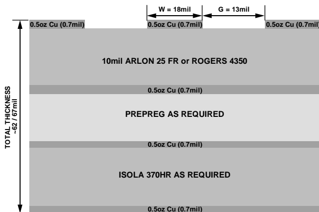
Figure 94. Evaluation Board Cross Sectional View
