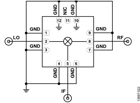
Figure 97. EV1HMC774ALC3B Evaluation Board Schematic
