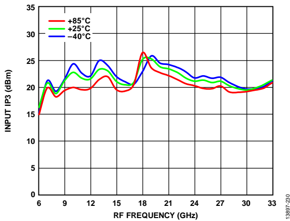
Figure 30. Input IP3 vs. RF Frequency over Various Temperatures, P_{LO} = 15 dBm
