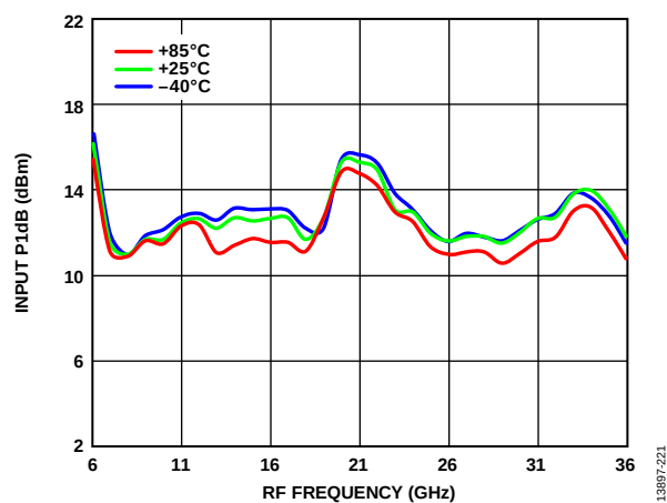
Figure 21. Input P1dB vs. RF Frequency over Various Temperatures, P_{LO} = 15 dBm
