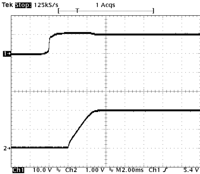
Fig-2.0V-4: Turn-on transient for V_{out}=2.0V with application of V_{in} at full rated load current (resistive) and 47uFx4 external capacitance at V_{in}=12V . Top trace: V_{in} (10V/div.) Bottom trace: output voltage (1V/div.) Time scale: 2 ms/div.
