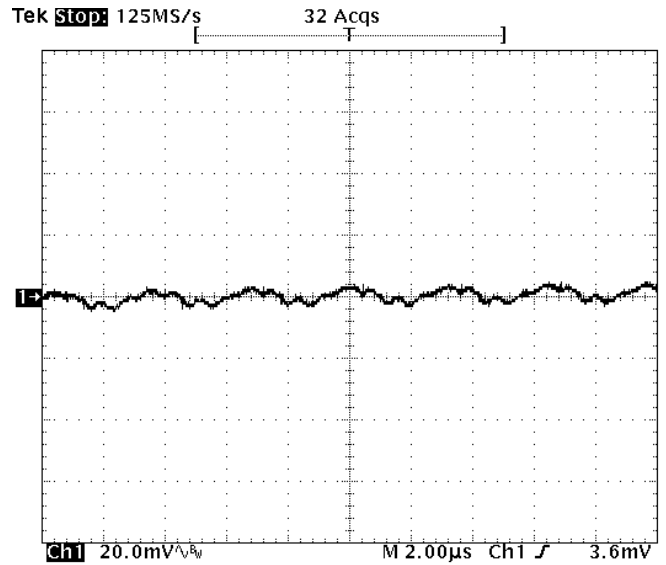
Fig-2.0V-5: Output voltage ripple (20mV/div.) for V_{out}=2.0V at full rated load current into a resistive load with external capacitance 47uFx4 ceramic + 1uF ceramic at V_{in}=12V . Time scale: 2 us/div
