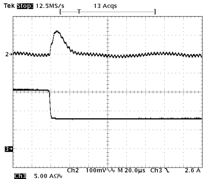
Fig-2.0V-7: Output voltage response for V_{out}=2.0V to negative load current step change from 16A to 8A with slew rate of -5A/us at V_{in}=12V . C_o=47uFx4 ceramic. Top trace: output voltage (100mV/div.) Bottom trace: load current (5A/div.) Time scale: 20us/div.
