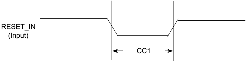
Figure 8. Reset Timing Diagram
